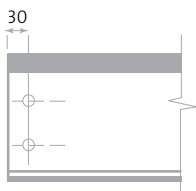
2 HOLES Ø18
